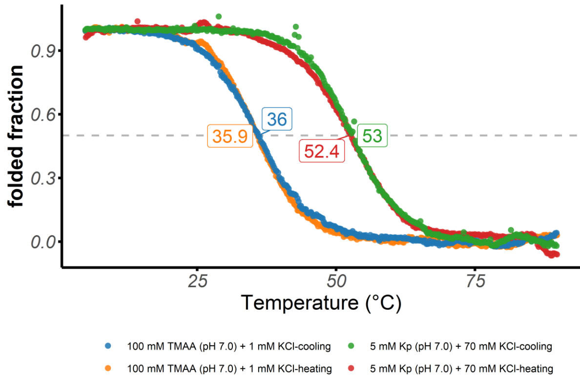
Folded fraction of the 5LQG oligonucleotide as a function of temperature, determined by UV-melting ( \lambda = 295 \text{ nm} )
