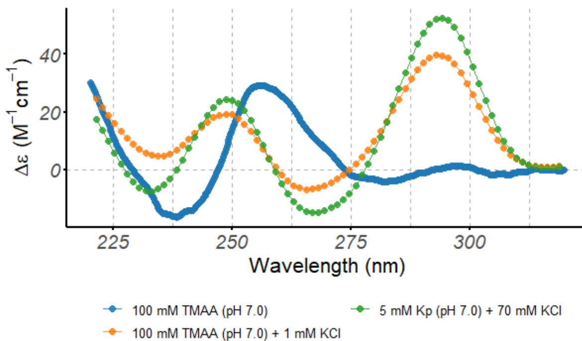
Circular dichroism spectra of the 5LQG oligonucleotide (10 \mu M), acquired at 25°C in 0.4-cm path-length cuvettes
